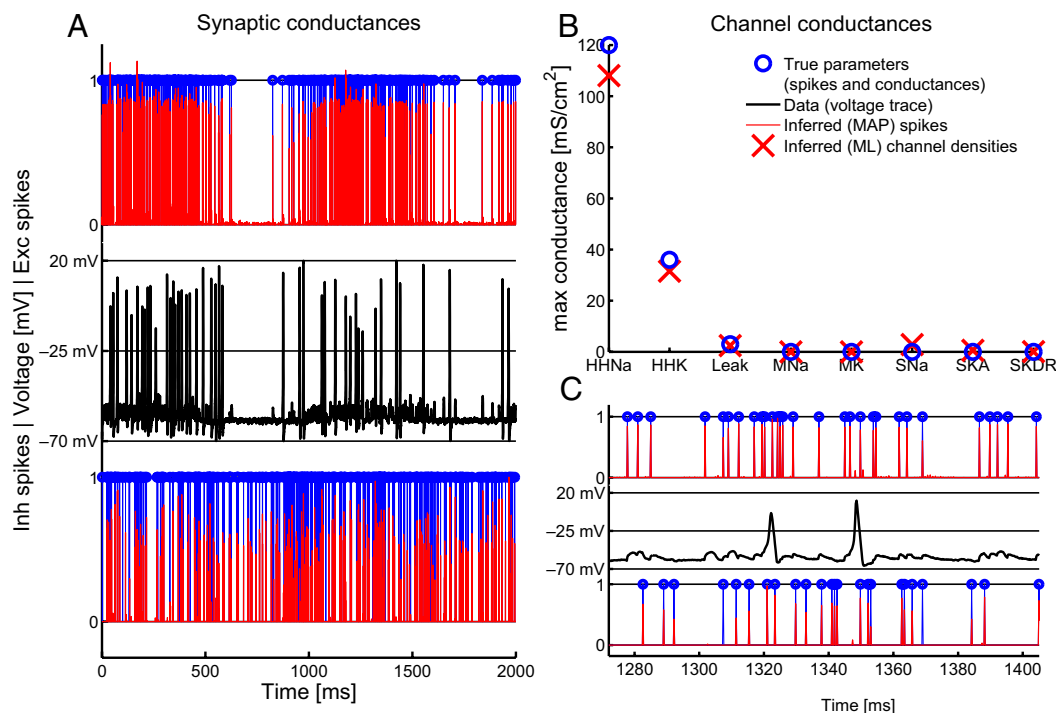
FIG. 15. Joint inference of synaptic input and channel densities. True parameters are in blue, the inferred parameters in red. A , top : excitatory synaptic input; middle : voltage trace (the only observed data); bottom : inhibitory synaptic input. B : true and inferred channel densities; channels are the same as in INFERRING CHANNEL CONDUCTANCES IN A MULTICOMPARTMENT MODEL. C : same data as A but magnified. Note that the channel densities are inferred well and that all excitatory spikes are correctly inferred, but a few inhibitory spikes are missed when the voltage is too close to the reversal potential of the inhibitory synapse.
