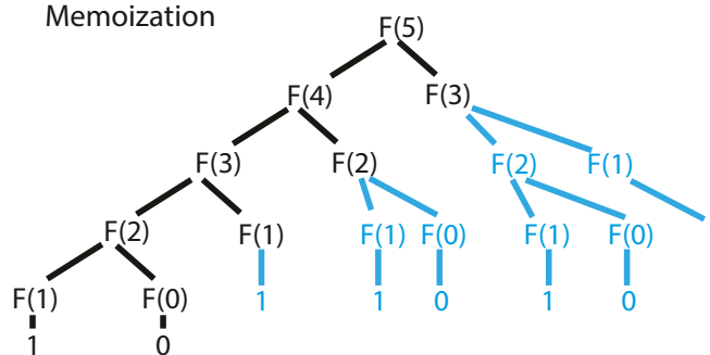
Fig. S6. Memoization. The Fibonacci number n is the sum of Fibonacci numbers n - 1 and n - 2 . The tree shows the computations required to compute the fifth Fibonacci number. If the lower Fibonacci numbers are stored instead of being recomputed on the fly every time they are required, then the part of the tree in blue does not need to be traversed, resulting in an exponential reduction of computational cost. Adapted from ref. 1.
