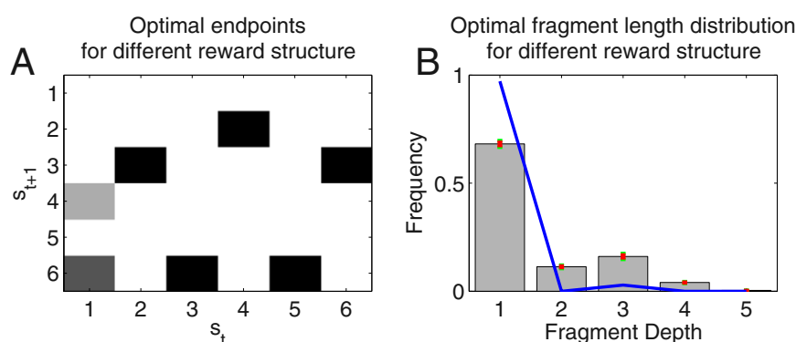
Fig. S7. Optimal endpoint distribution for an altered reward matrix. The outcomes for transitions 1–2 and 3–6 were swapped (i.e., the large reward moved from the top transition to the transition going from the left to the right through the middle of the maze). This leads to substantial changes in the optimal fragmentation endpoint pattern, shown in A , and to the distribution of fragment lengths, shown in B as a blue line superimposed on the fragment length distribution inferred from the data (replotted from Fig. 3).
